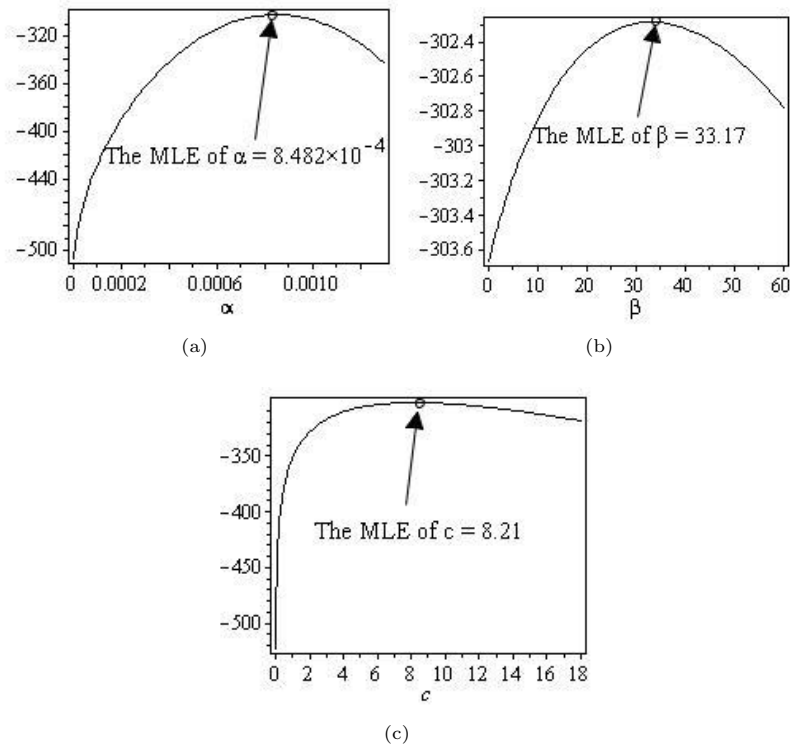
Figure 8. For Abuammoh et al data, (a) The profile of log-likelihood function of \alpha . (b) The profile of log-likelihood function of \beta . (c) The profile of log-likelihood function of c .
