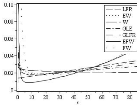
Figure 4. The fitted hazard functions of selected models for Aarset data.
