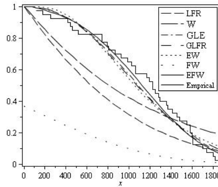
Figure 6. The empirical and fitted survival functions of selected models for Abuammoh et al data.
