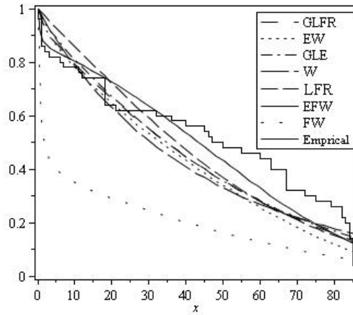
Figure 3. The empirical and fitted survival functions of selected models for Aarset data.
