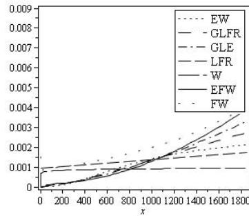
Figure 7. The fitted hazard functions of selected models for Abuammoh et al data.
