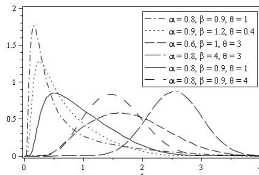
Figure 1. The pdf of the EFW distribution at different values of its parameters
