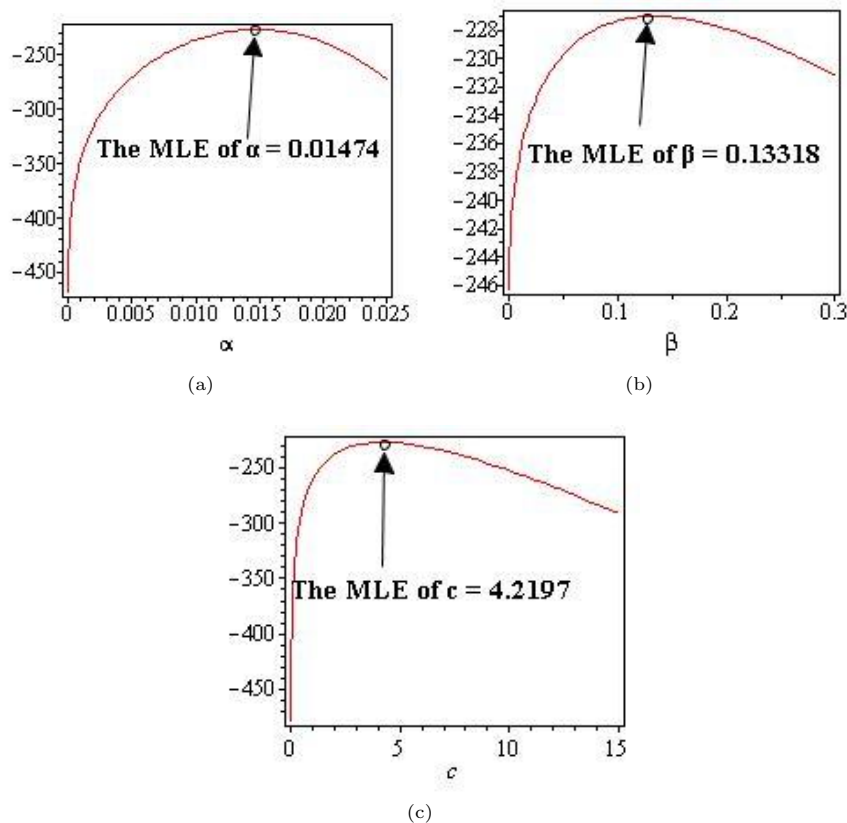
Figure 5. For Aarset data, (a) The profile of log-likelihood function of \alpha . (b) The profile of log-likelihood function of \beta . (c) The profile of log-likelihood function of c .
