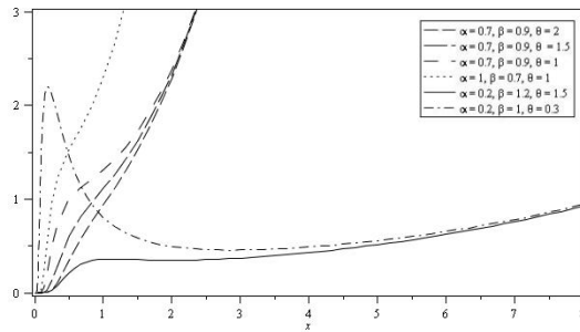
Figure 2. The hazard function of the EFW distribution at different values of its parameters.
